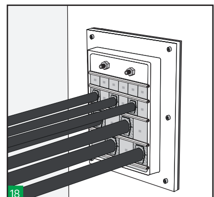
18 Make a visual inspection of the transit. Hawke's colour coding enables the installation to be visually inspected after completion and ensures correct matching of the blocks halves.
