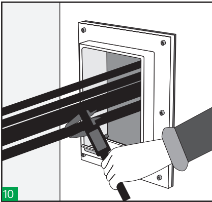
10 Take measures of the cables diameter with a calibre and select the appropriate Hawke tolerant blocks. Colour code will help you to select the correct ones. Only use H-DM black blocks.
